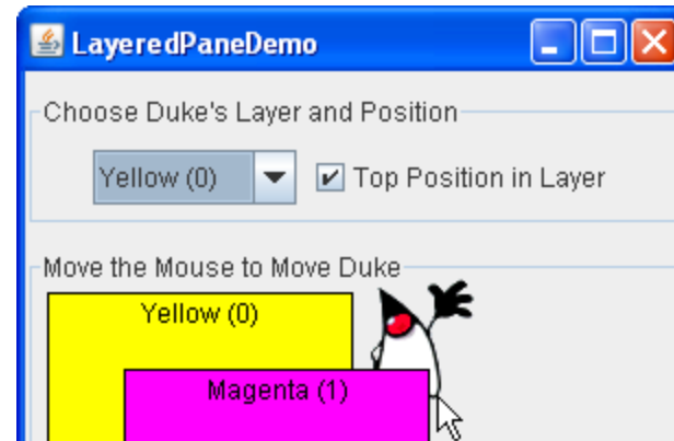
JLayeredPane
